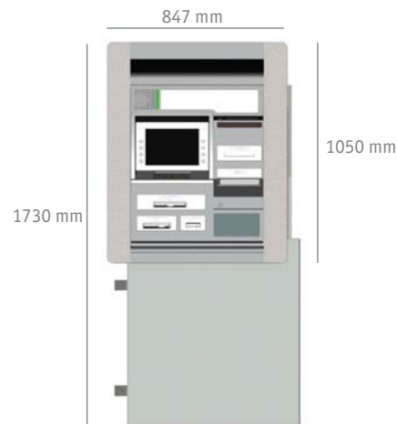
Dimensions shown are for Cash Star 7225, through-the-wall installation Weight: 950 kg
